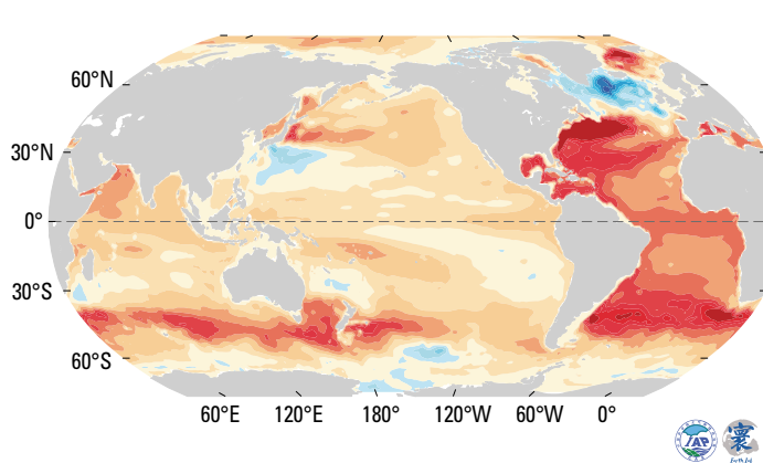
Figure 5. Observed upper 2000 m OHC trend from 1958 to 2023.
